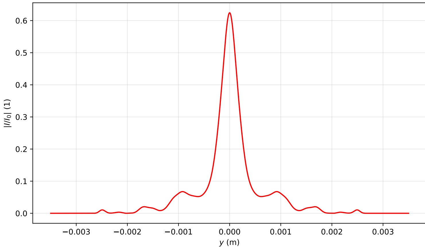
Intensity profile I(x = 0, y, z = 2.627)/I_0 , \text{Pin}=5.0\text{Pcr} , artificial time
